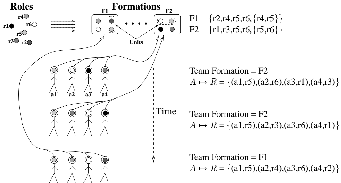
Figure 3: A team of agents smoothly switching roles and formations over time. Different roles are represented as differently shaded circles. Formations are possibly overlapping collections of roles. Units within the formations are indicated within a dotted enclosure. The definitions of all roles, formations, and units are known to all agents. An agent's current role is indicated by the shaded circle in its head and its current formation is indicated by an arrow to the formation. The agents first switch roles while staying in the same formation; then they switch to an entirely new formation.
