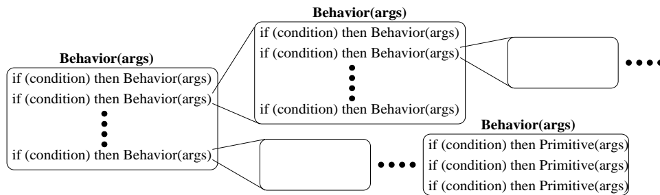
Figure 2: Behaviors in the team member agent architecture. Both internal and external behaviors are organized as directed acyclic graphs.
